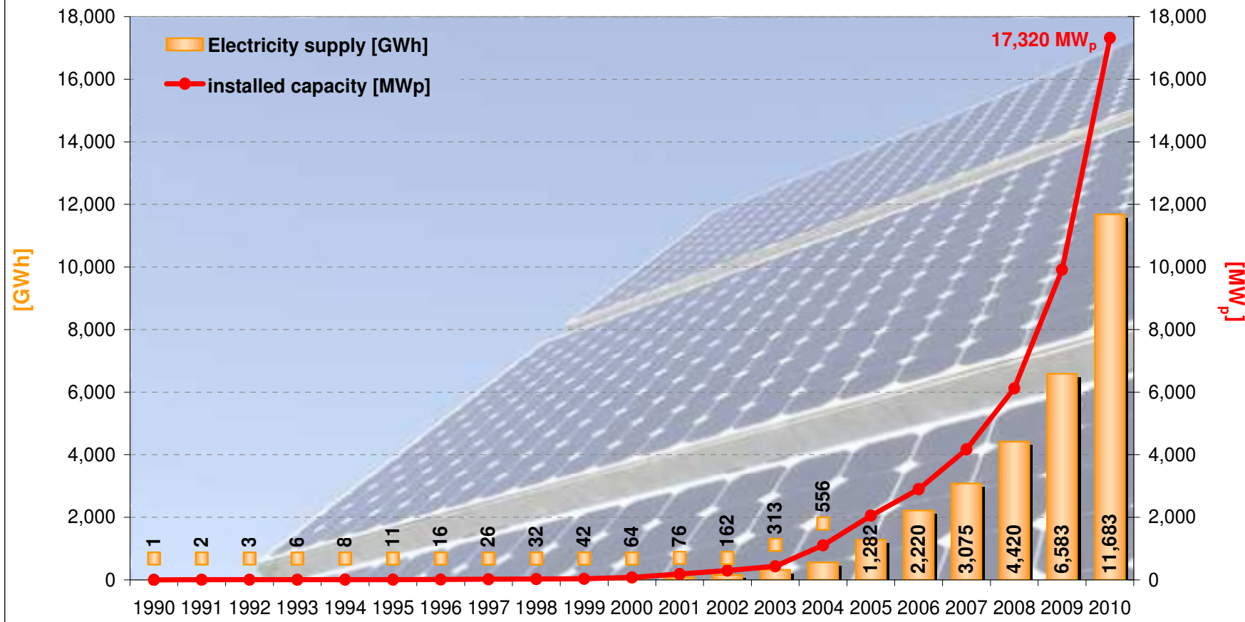
Installed capacity and electricity supply from photovoltaic installations in Germany
