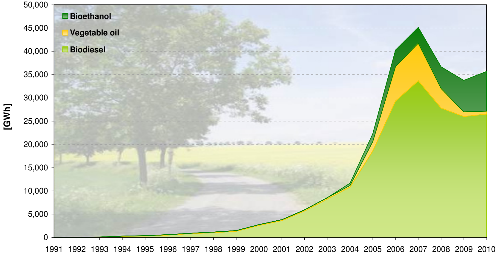
Contribution of renewable energy sources to fuel supply Germany
