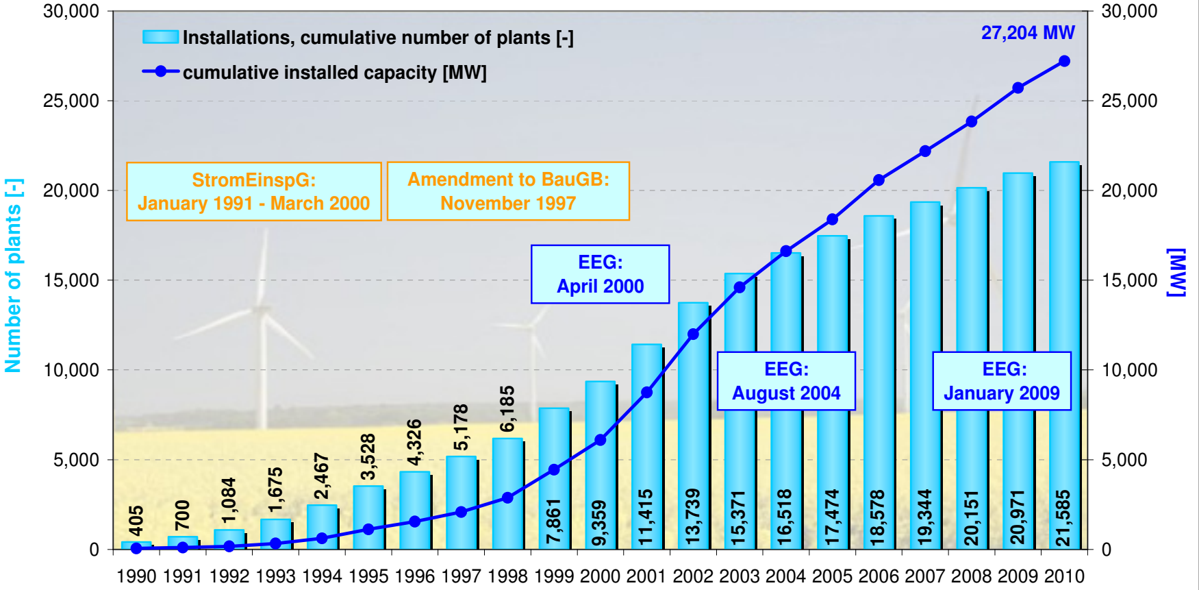
Development of the number and cumulative capacity of wind energy plants in Germany
